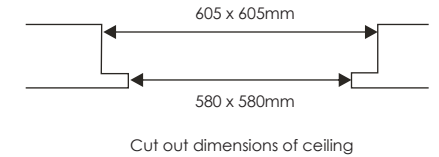
Cut out dimensions of ceiling
