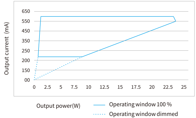
Operating window
