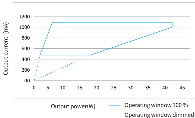
Operating window
